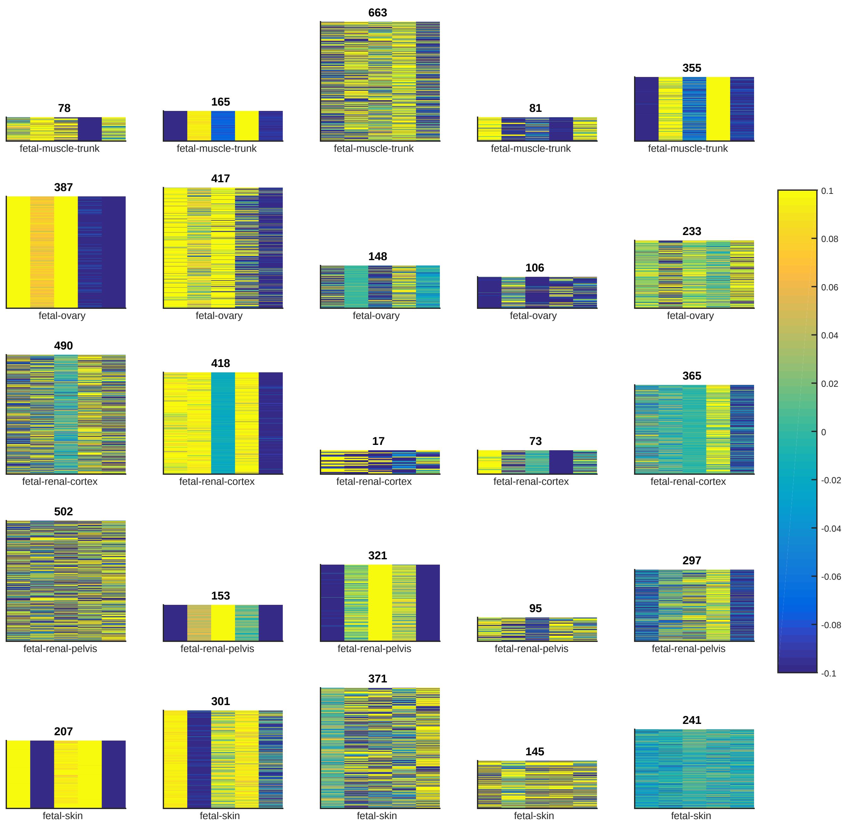
Plot of Arboretum output clusters for k=5 and random initialization 1; Autismspectrumdisorderorschizophrenia.5
