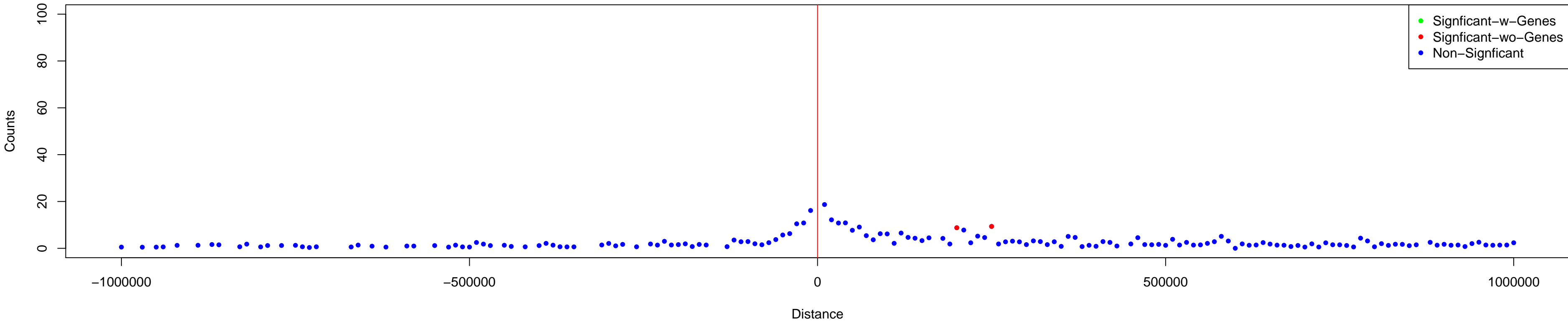
Gould_HiC_Data chr5_80330000_80340000
