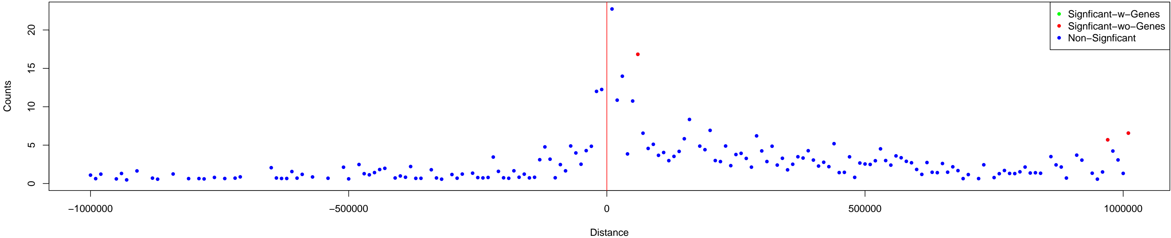
Gould_HiC_Data chr5_80330000_80340000
