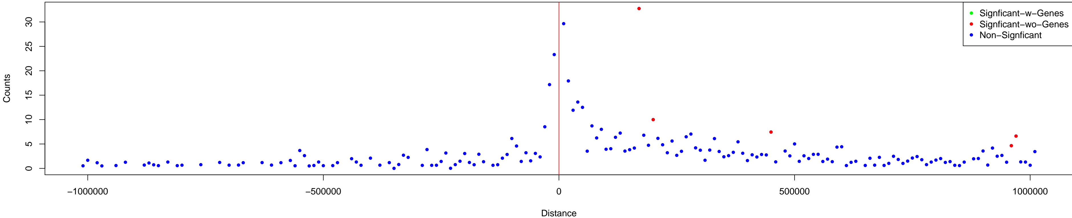
Gould_HiC_Data chr5_80330000_80340000
