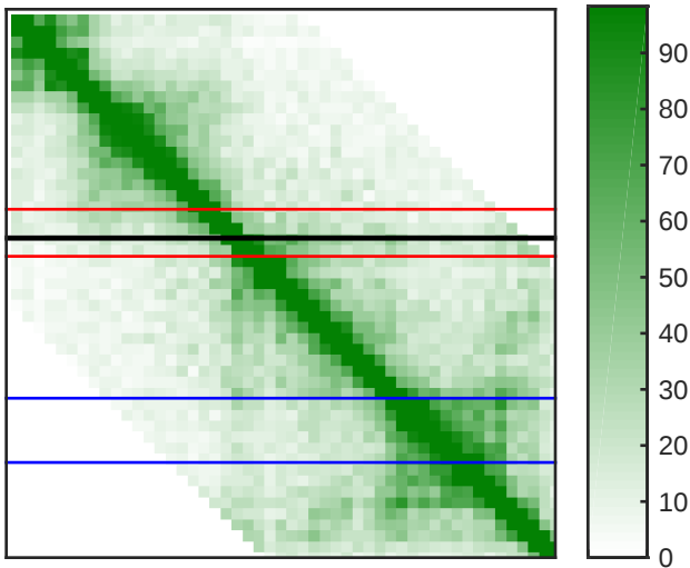
44-loop-12wk-dna
